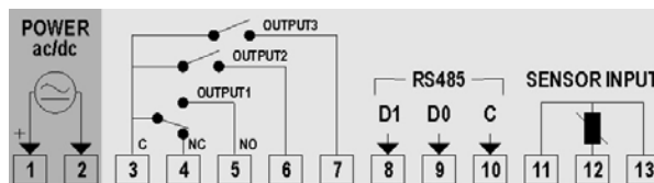
Figure 1 – Bornier N323
